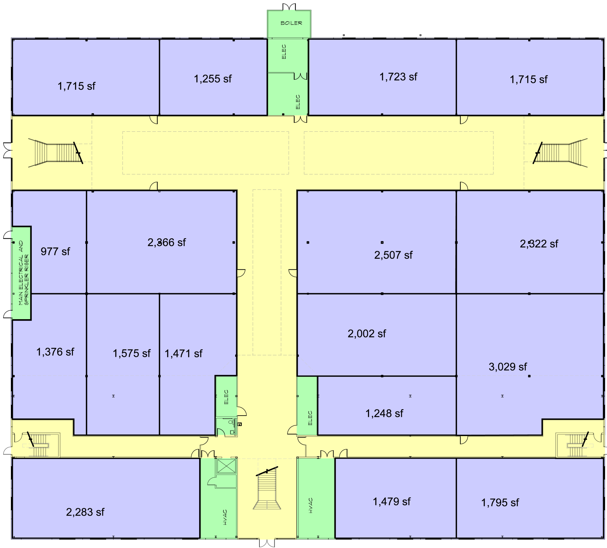
FIRST FLOOR PLAN SCALE: NTS
